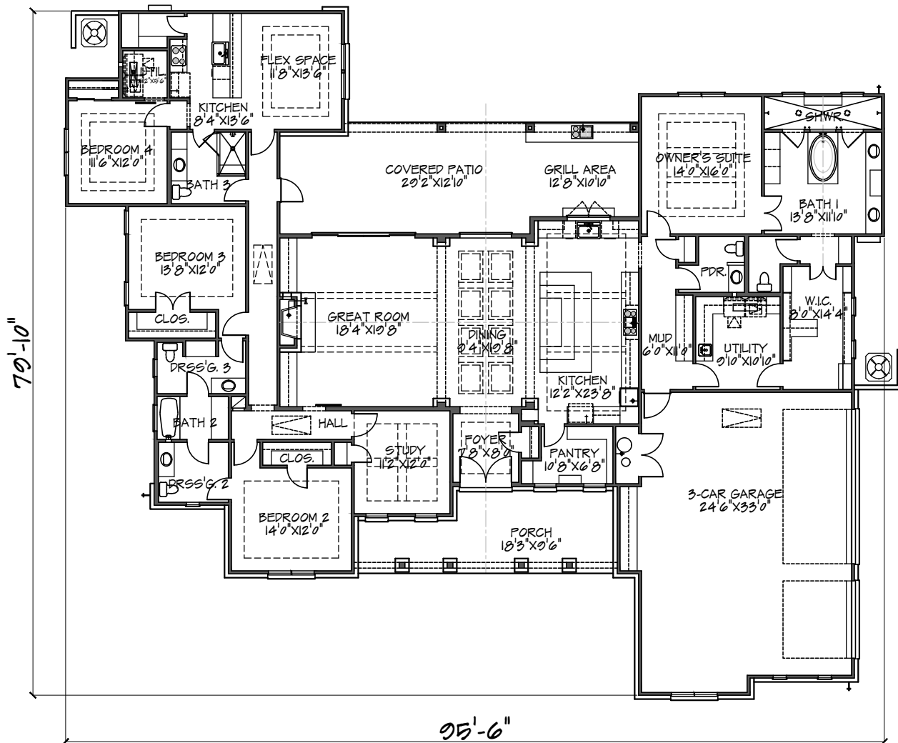
FLOOR PLAN 3,892 SQ. FT.
